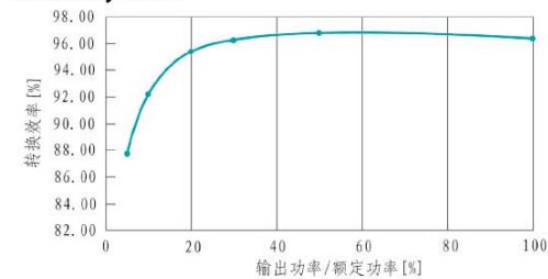
Efficiency curve
