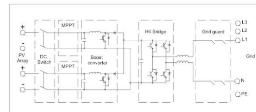
Electrical drawing
